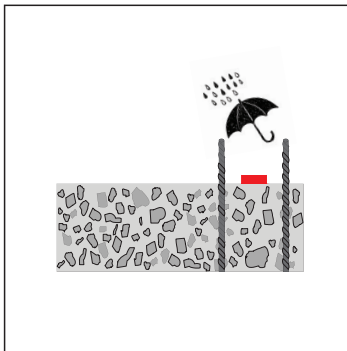
Protect swelling gasket from wet and dirt
